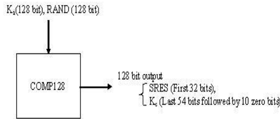
Figure 2.2: COMP 128 Calculations
