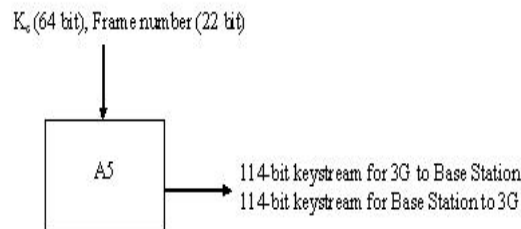
Figure 2.3: Keystream Generations
