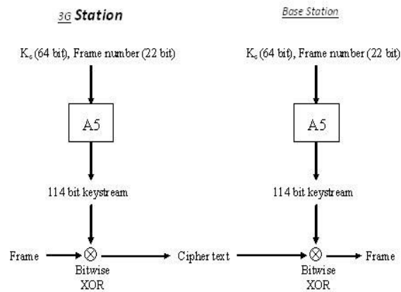
Figure 2.4: Frame Encryption and Decryption
