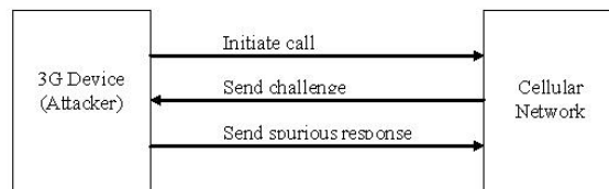
Figure 3.3: DoS by Spurious Authentication
