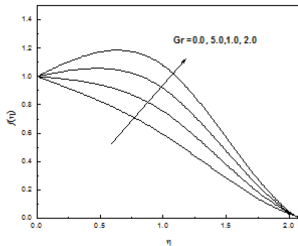
Figure-1: Velocity Profiles for Different Values of Gr
