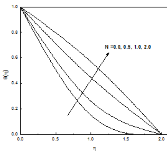
Figure-10: Temperature Profiles for Different Values of N
