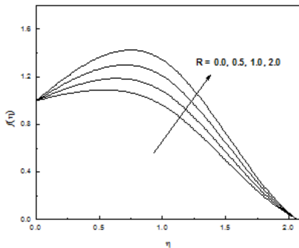
Figure-7: Velocity Profiles for Different Values of R
