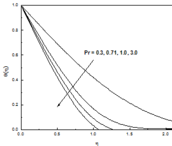
Figure-6: Temperature Profiles for Different Values of Pr
