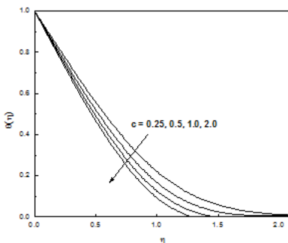
Figure-14: Temperature Profiles for Different Values of c
