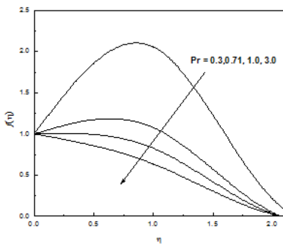
Figure-5: Velocity Profiles for Different Values of Pr
