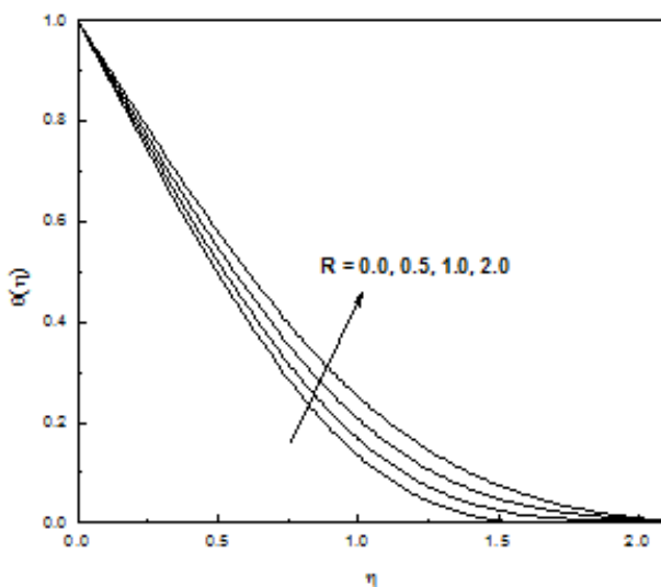
Figure-8: Temperature Profiles for Different Values of R
