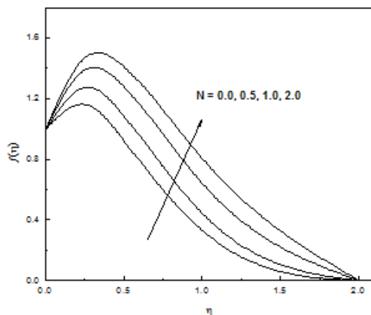
Figure-9: Velocity Profiles for Different Values of N
