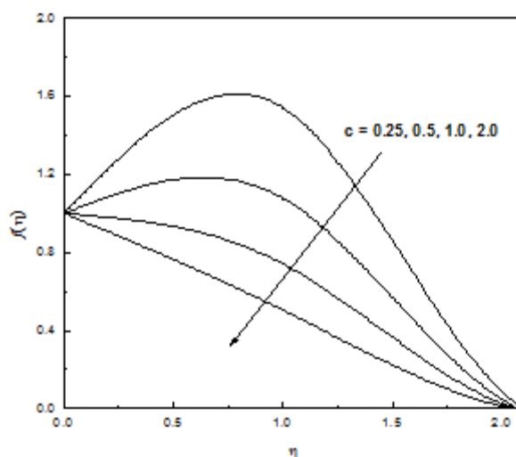
Figure-13: Velocity Profiles for Different Values of c
