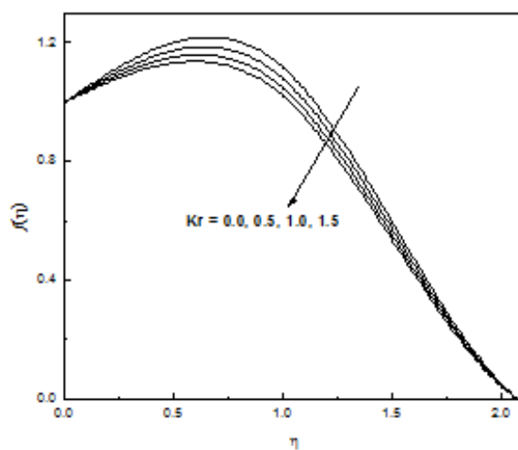
Figure-11: Velocity Profiles for Different Values of Kr
