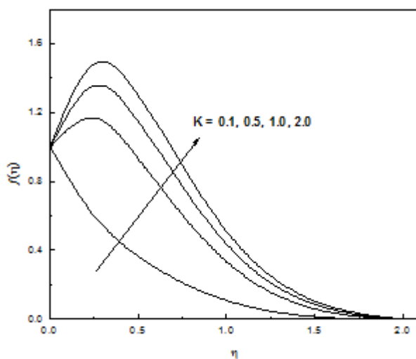
Figure-4: Velocity Profiles for Different Values of K
