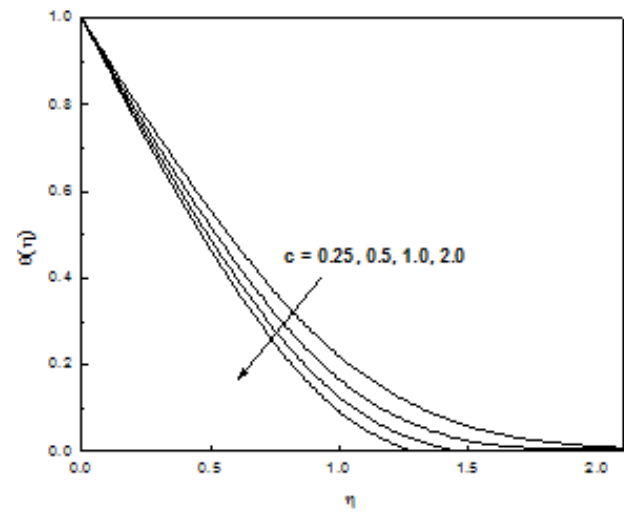
Figure-14: Temperature Profiles for Different Values of c
