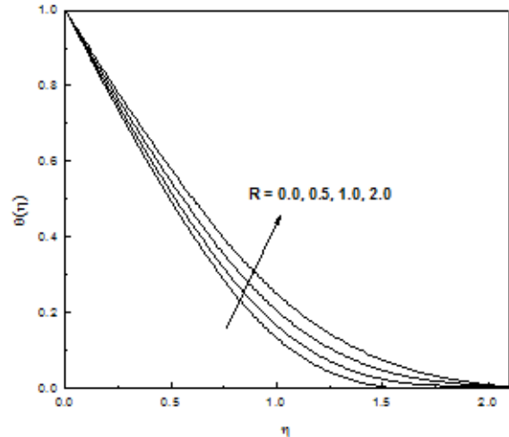
Figure-8: Temperature Profiles for Different Values of R
