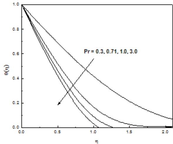
Figure-6: Temperature Profiles for Different Values of Pr
