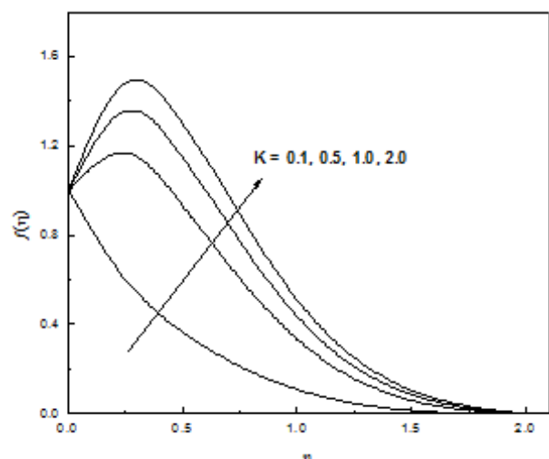
Figure-4: Velocity Profiles for Different Values of K
