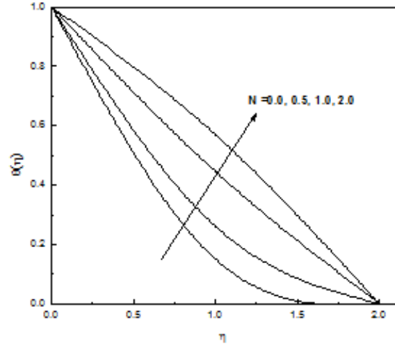
Figure-10: Temperature Profiles for Different Values of N
