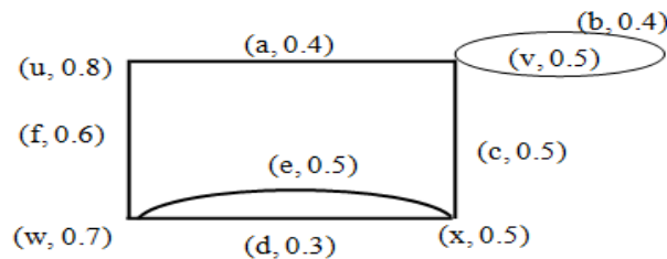
Figure-2.1: Fuzzy graph F
