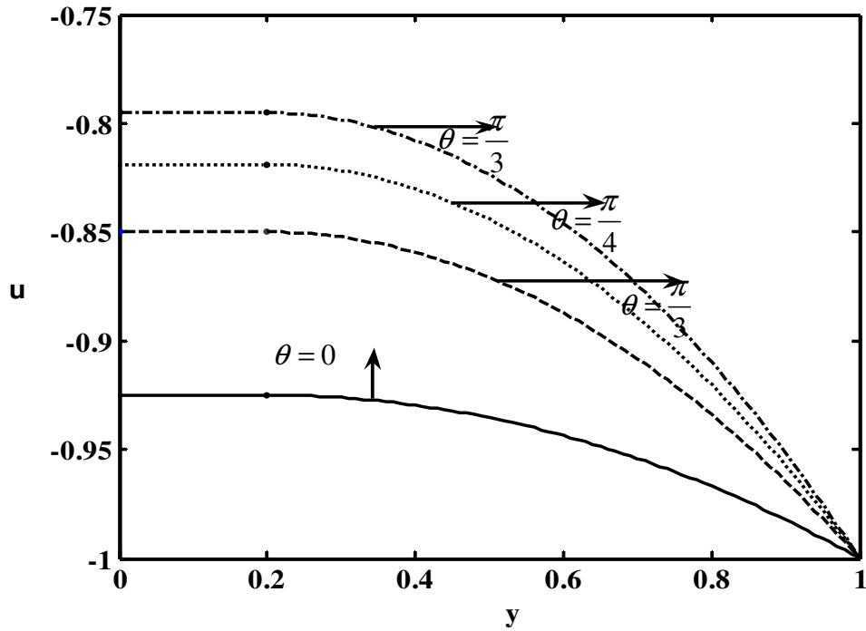
Fig. 2(ii) The variation of axial velocity u with y at x = 0.25 for different values of inclination angle \theta with \phi = 0.6, M = 0.5, \eta_1 = 0.5, y_0 = 0.2 and for \frac{\partial p}{\partial x} = 0 .
