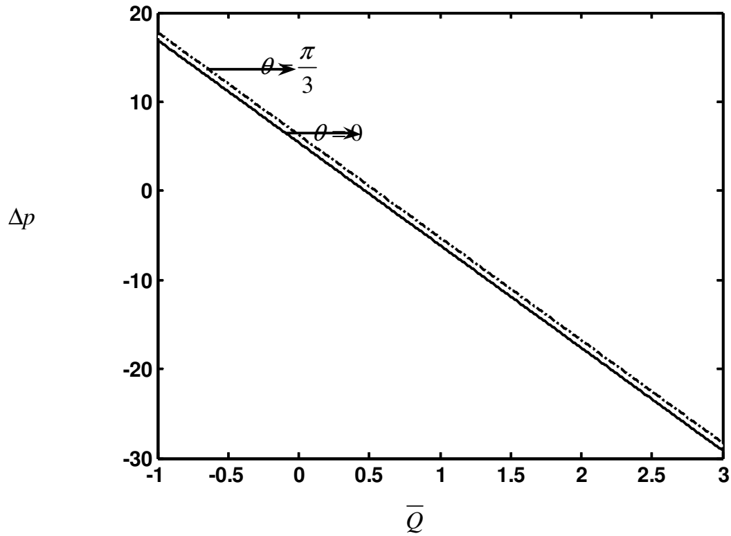
Fig. 5 The variation of pressure rise \Delta p with average volume flow rate \bar{Q} for different values of \theta with \phi = 0.6, y_0 = 0.01, M = 0.5, and \eta_1 = 1 .
