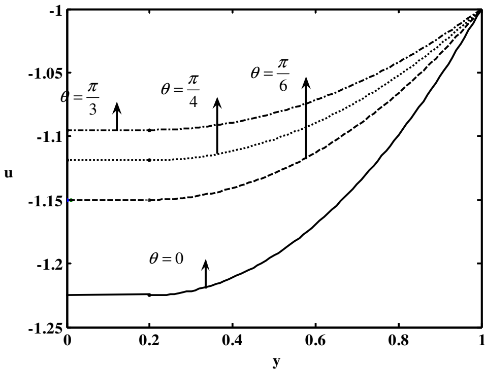
Fig. 2(iii) The variation of axial velocity u with y at x = 0.25 for different values of inclination angle \theta with \phi = 0.6, M = 0.5, \eta_1 = 0.5, y_0 = 0.2 and for \frac{\partial p}{\partial x} = 1 .
