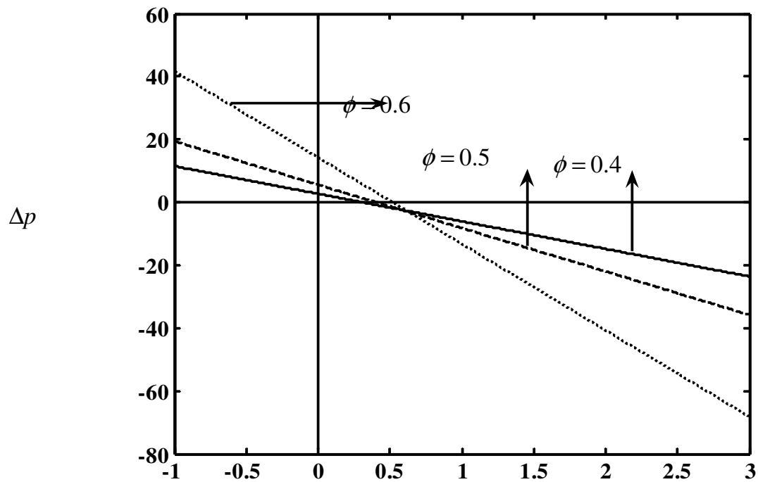
Fig. 6 The variation of pressure rise \Delta p with average volume flow rate \bar{Q} for different values of \phi with \theta = \pi/4, y_0 = 0.2, M = 0.5, and \eta_1 = 0.5 .
