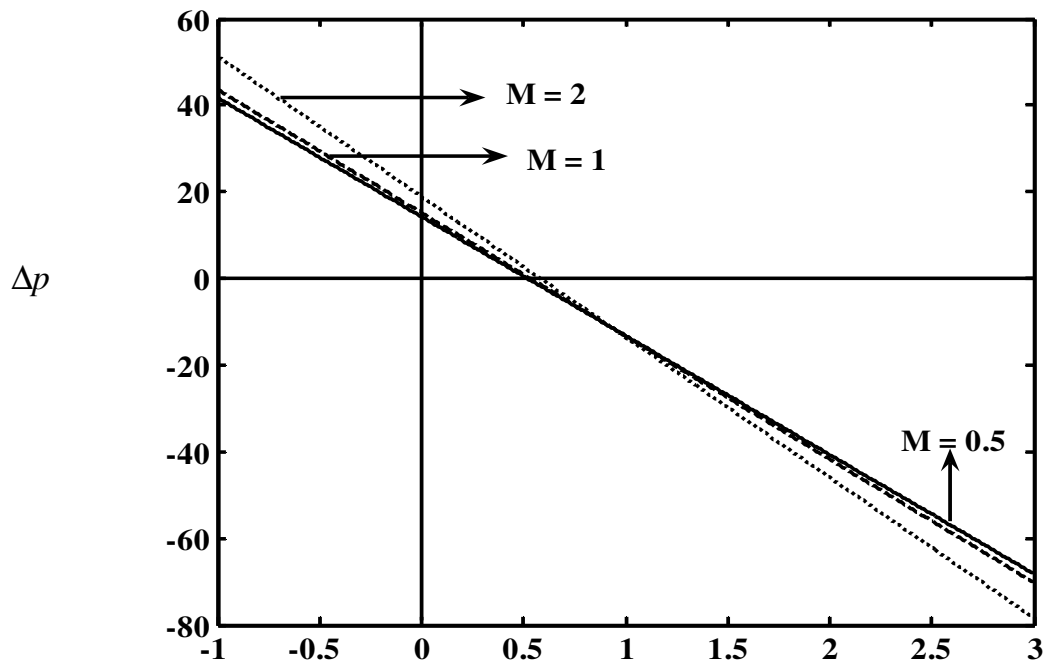
Fig. 4 The variation of pressure rise \Delta p with average volume flow rate \bar{Q} for different values of M with \phi = 0.6, y_0 = 2, \theta = \pi/4 , and \eta_1 = 0.5 .
