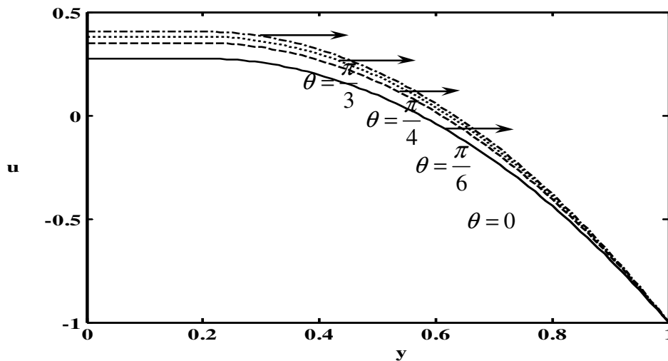
Fig. 2(i) The variation of axial velocity u with y at x = 0.25 for different values of inclination angle \theta with \phi = 0.6, M = 0.5, \eta_1 = 0.5, y_0 = 0.2 and for \frac{\partial p}{\partial x} = -4 .
