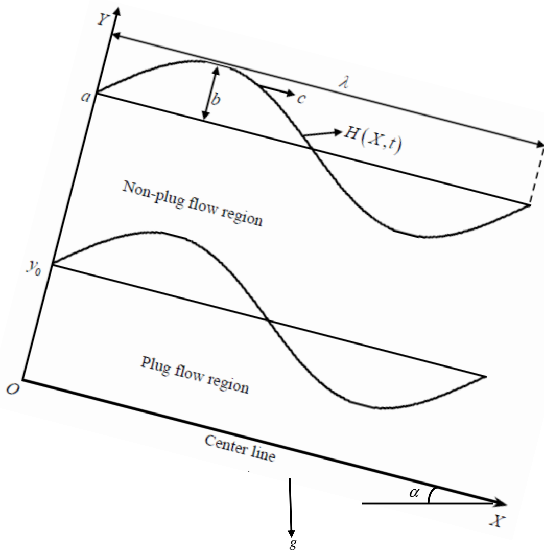
Fig. 1 The Physical model
