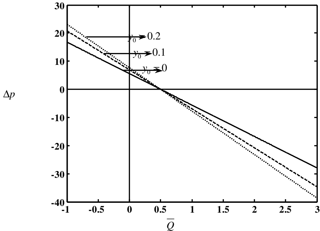
Fig. 7 The variation of pressure rise \Delta p with average volume flow rate \bar{Q} for different values of y_0 with \theta = \pi/4, \phi = 0.6, M = 0.5 , and \eta_1 = 0.5 .
