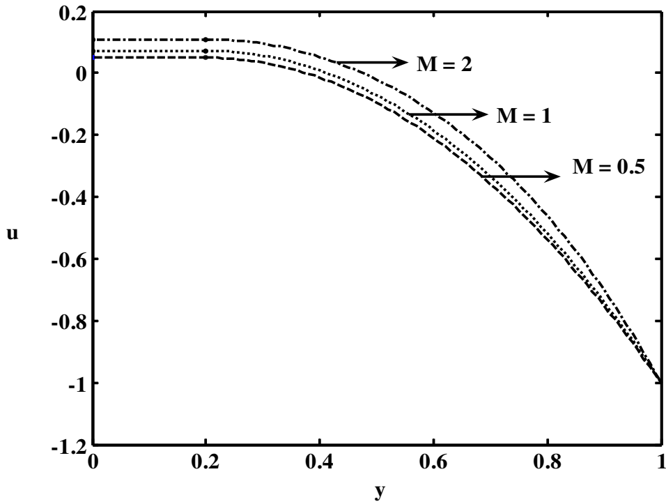
Fig. 3(i). The variation of axial velocity u with y at x = 0.25 for different values of Hartmann number M with \phi = 0.6, \theta = \pi/6, \eta_1 = 0.5, y_0 = 0.2 and for \frac{\partial p}{\partial x} = -3 .
